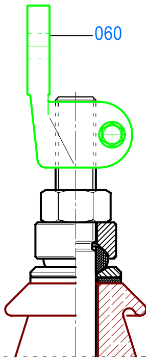
Option with flag for 1kV - 630A
